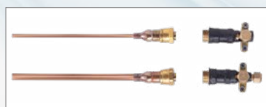
Quick-Connection – quick and easy installation of the system by means of „Plug & Play“ coupling connectors (except CL 6044 CB)
